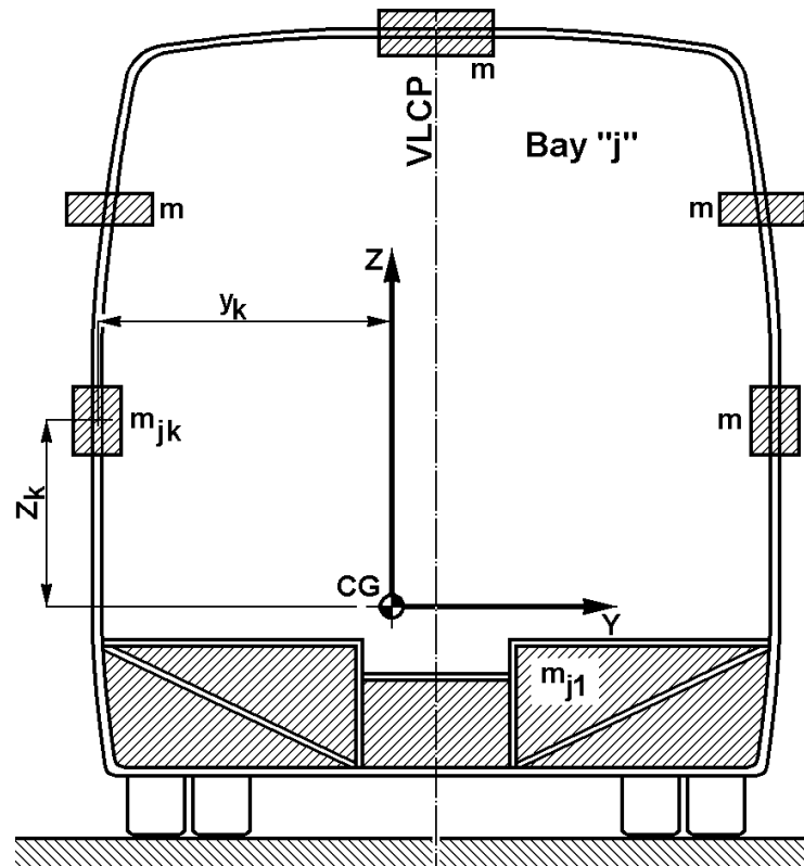
Figure A4.4 - Distribution of mass in the cross section of a bay
