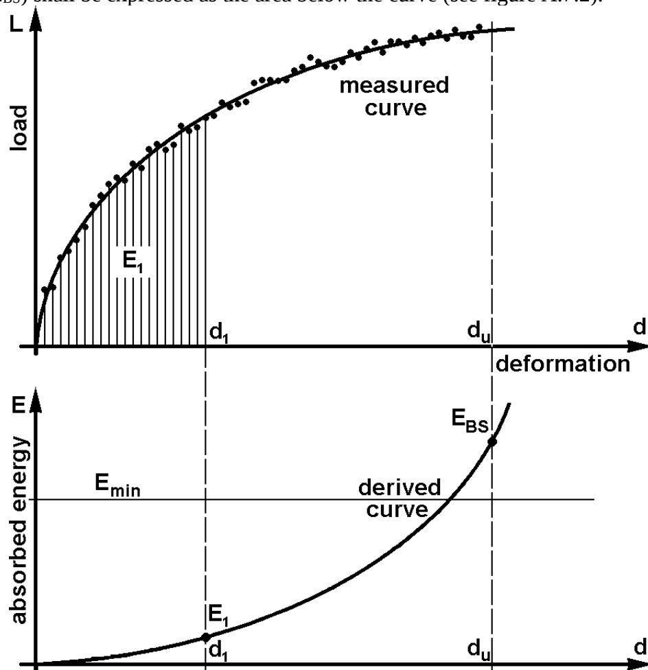
Figure A7. 2 - Absorbed energy for the body section, derived from the measured load-deformation curve
